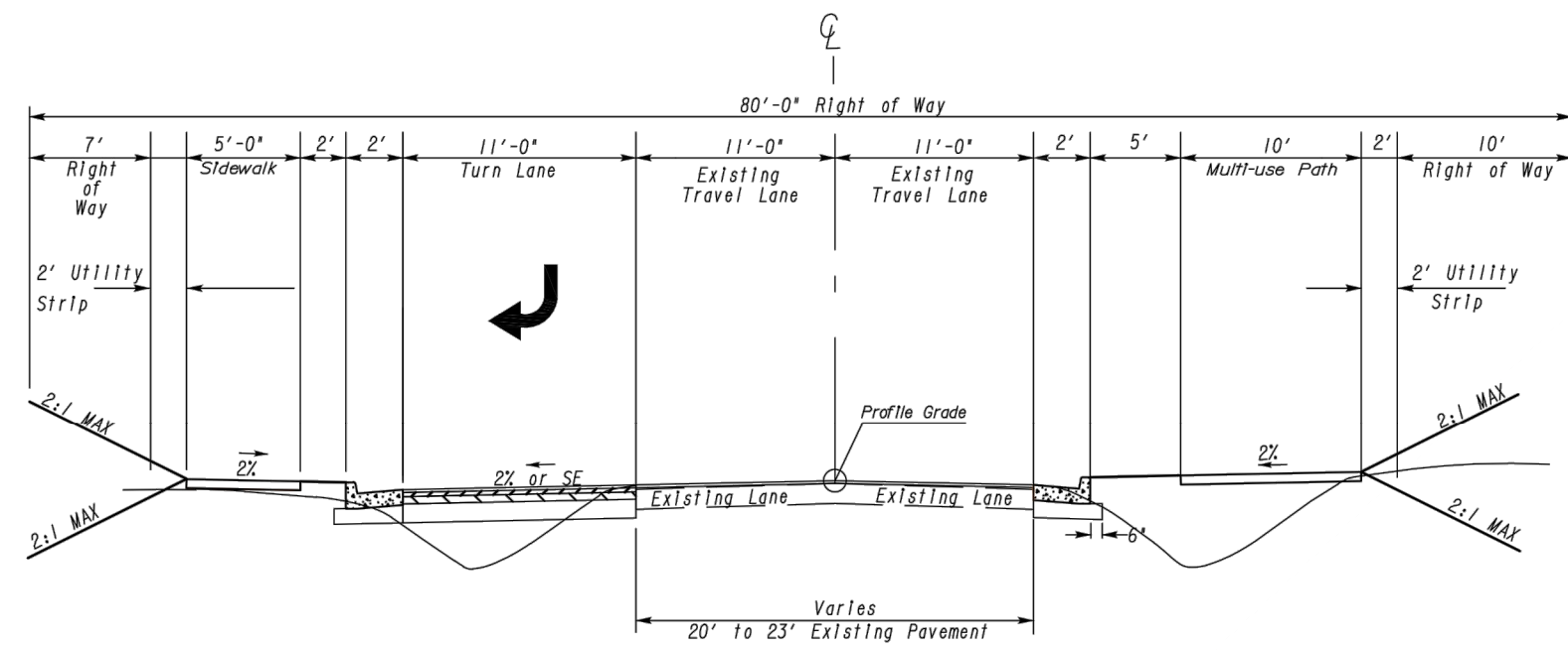
TYPICAL OVERLAY / WIDENING SECTION ASHFORD DUNWOODY ROAD NOT TO SCALE DESIGN SPEED = 40 MPH e max = 0.06
