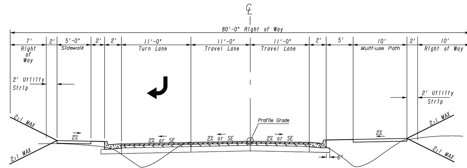
TYPICAL OVERLAY / WIDENING SECTION ASHFORD DUNWOODY ROAD NOT TO SCALE DESIGN SPEED = 40 MPH e max = 0.06
