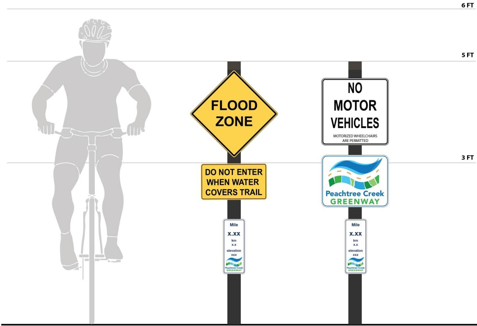
FRONT VIEW
