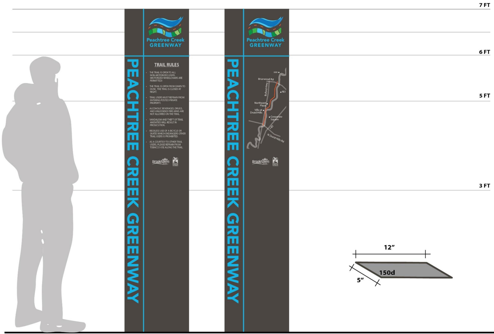
FRONT VIEW
