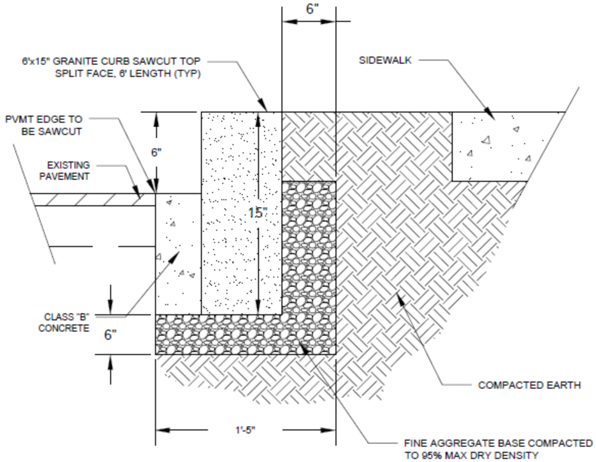
6" GRANITE CURB DETAIL SCALE: NTS
