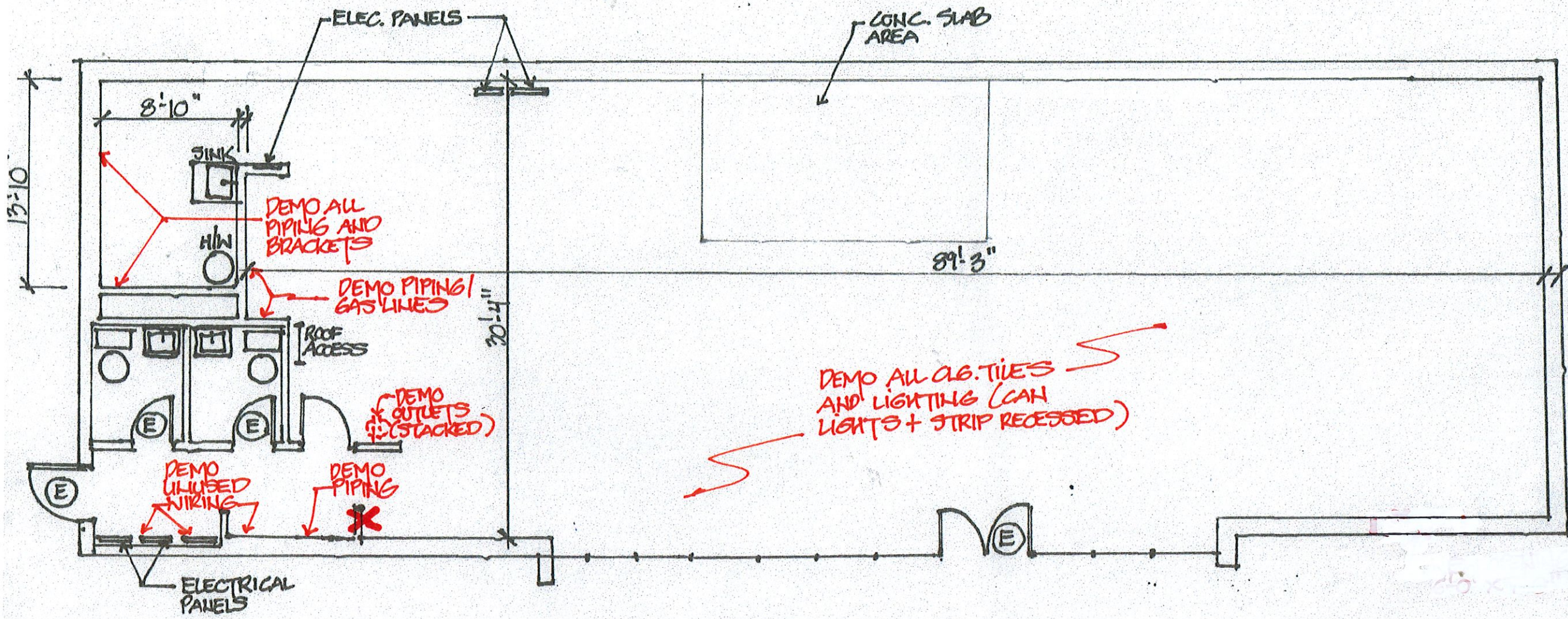
① EXISTING CONDITIONS / DEMOLITION PLAN SCALE: 1/8" = 1'-0"
