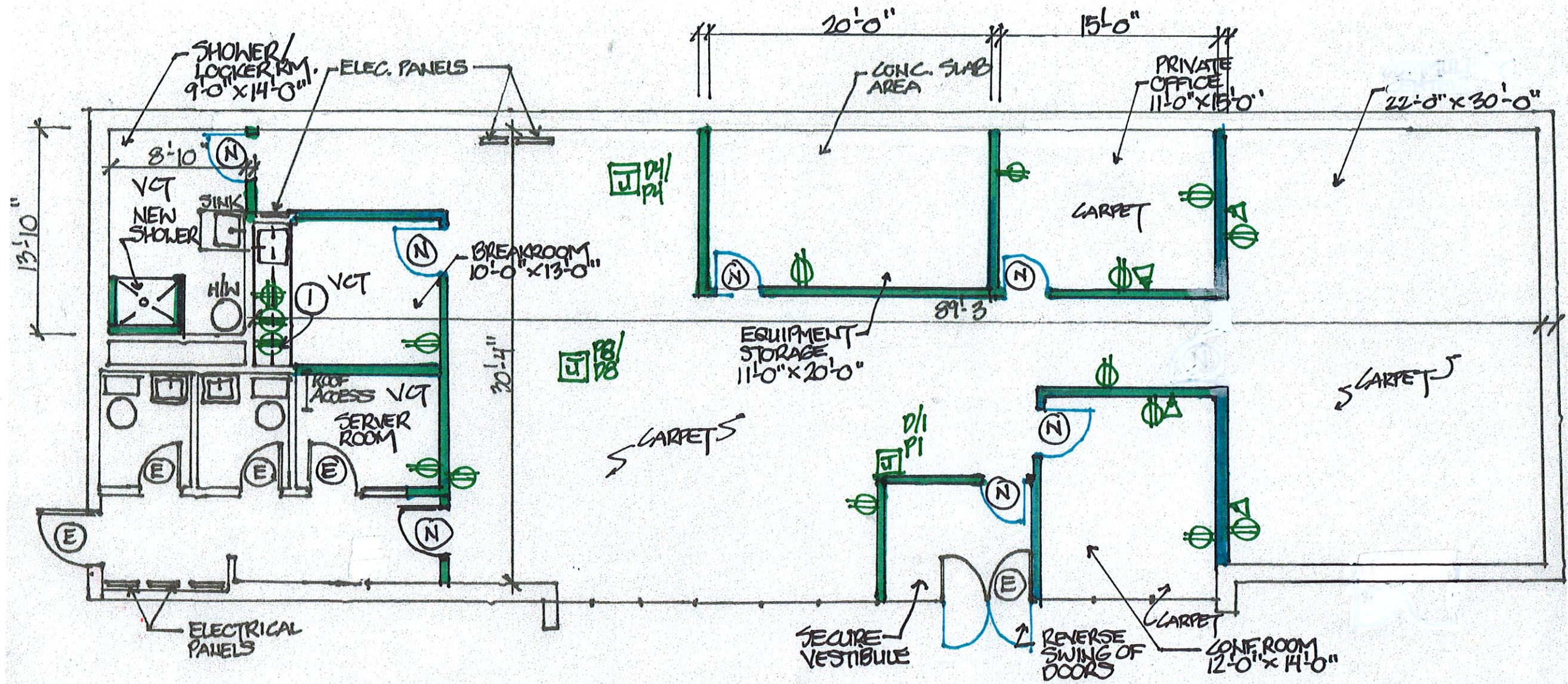
2 CONSTRUCTION FLOOR PLAN SCALE: 1/8" = 1'-0"
