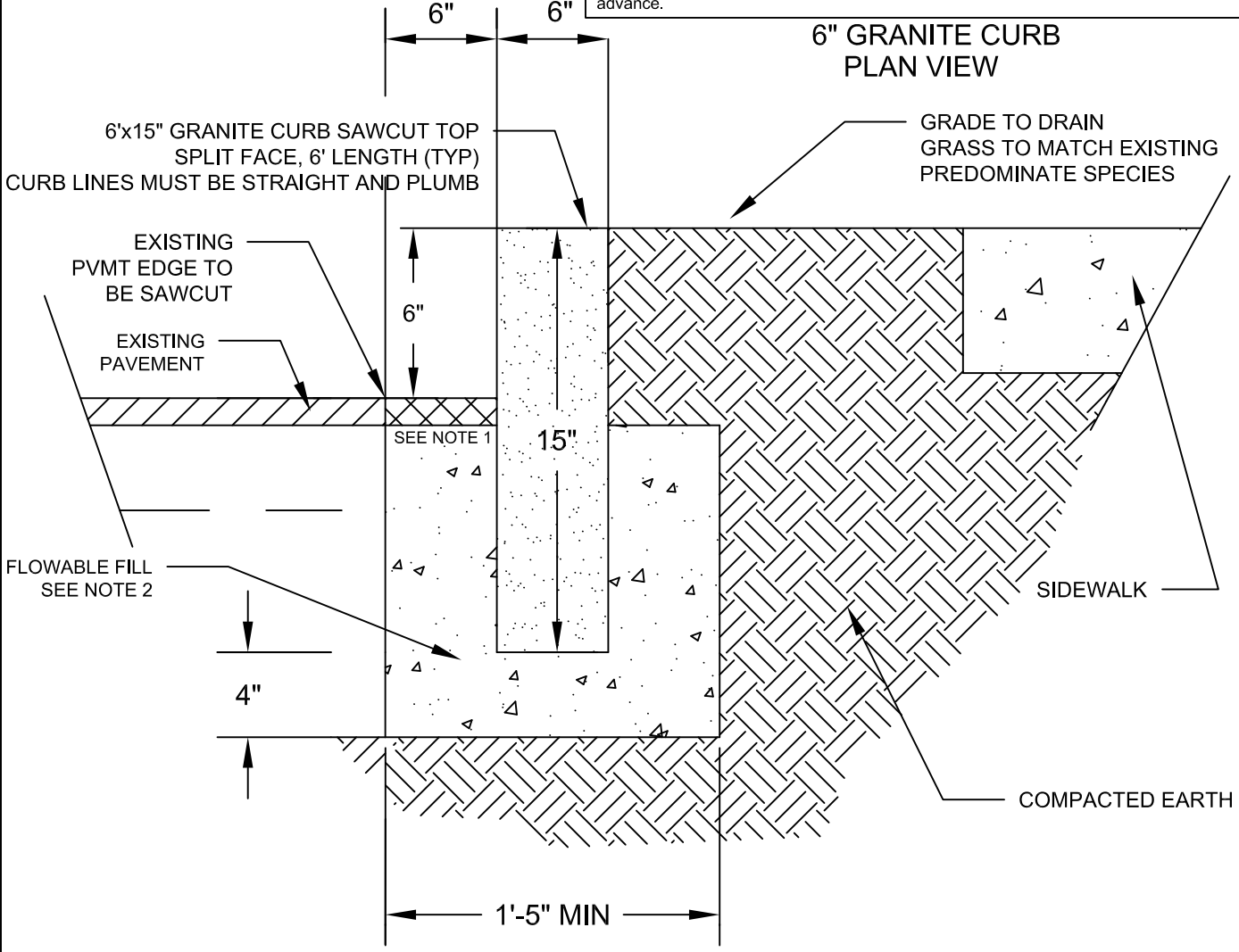
6" GRANITE CURB DETAIL
