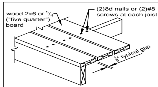
FIGURE 1: TYPICAL DECKING
